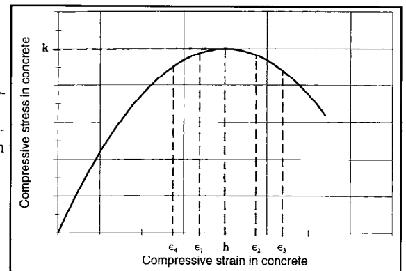
Figure 1 Parabolic stress-strain curve for concrete in compression with examples of measured strain values at peak load on the specimen
