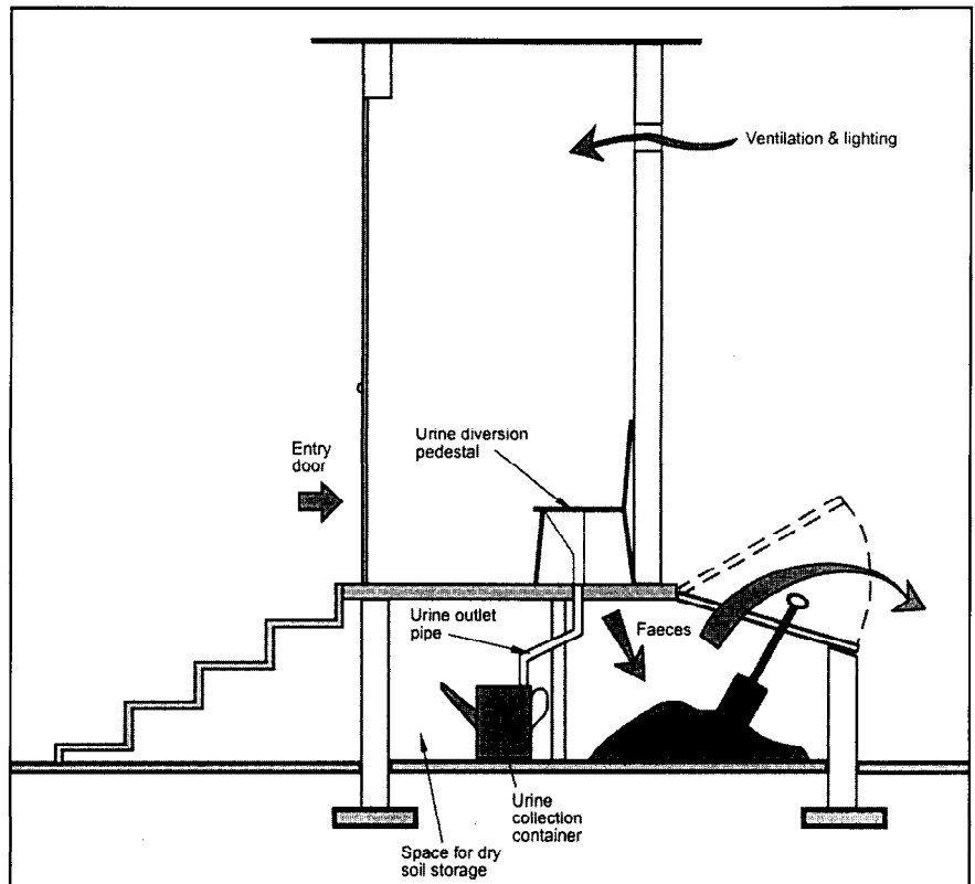
Figure 1 Schematic representation of a urine diversion ('dry-box') toilet
