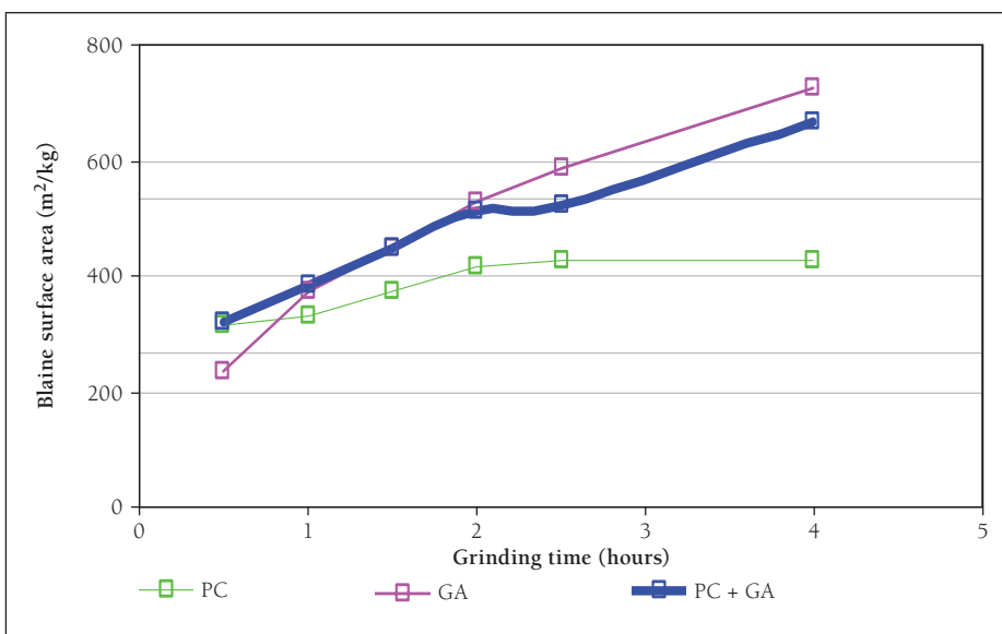
Figure 9 Graph indicating Blaine surface areas
